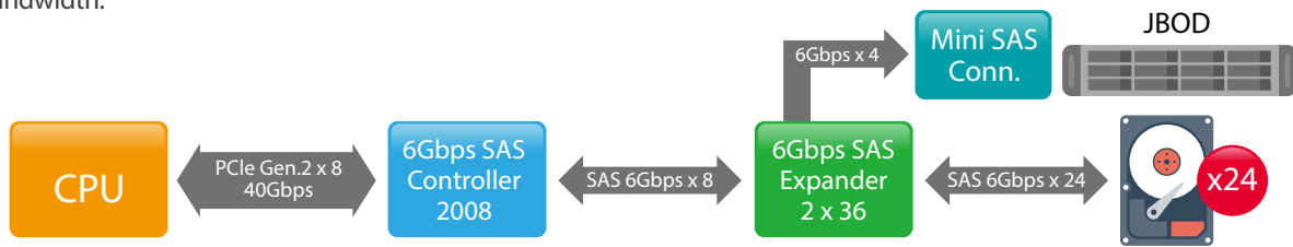
TS-x79U-SAS 6G SAS model block diagram
